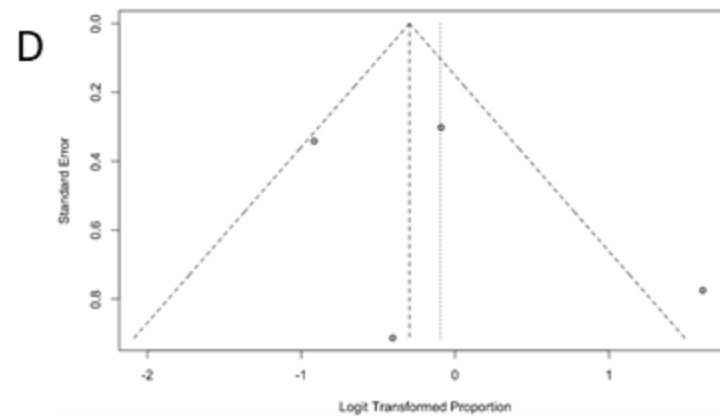
Funnel plot with pseudo 95% confidence limits
