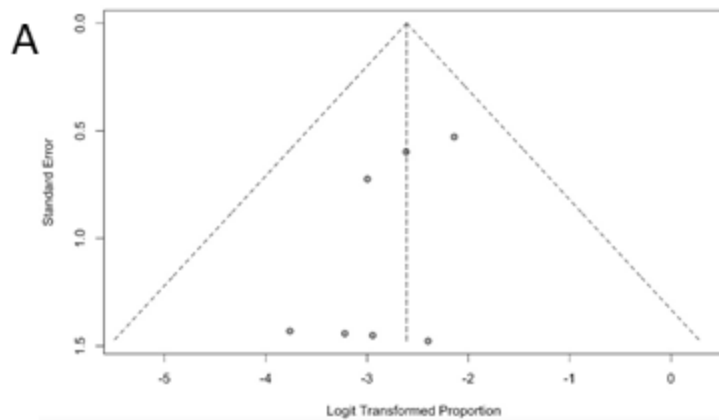
Funnel plot with pseudo 95% confidence limits
