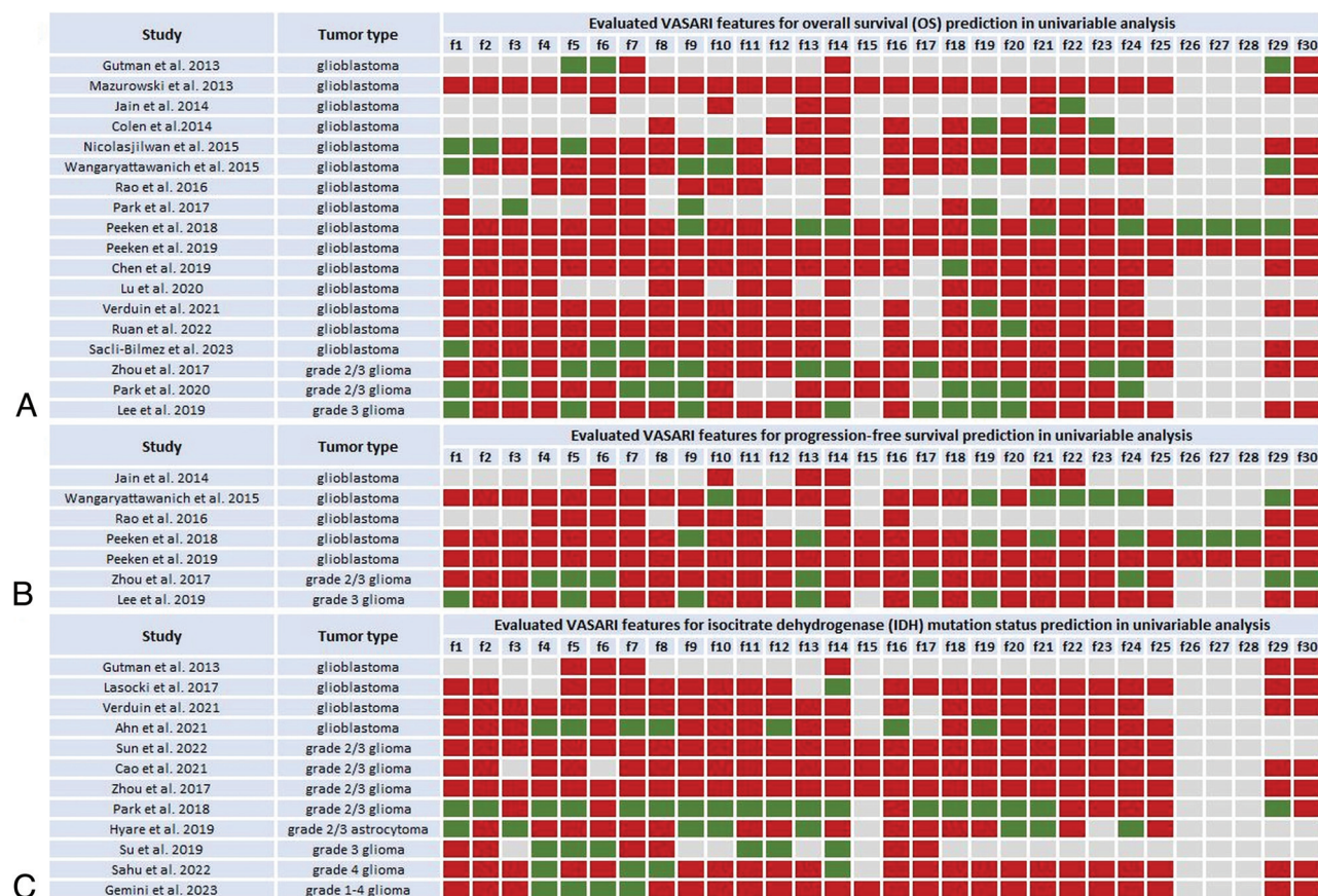
FIG 2. The association between different VASARI features and OS (A), progression-free survival (B), and IDH mutation status (C) listed per study involving glioblastoma and grades 1–4 glioma cohorts. Green indicates tested and significant feature; red, tested and nonsignificant feature or feature with statistical results not provided; gray, features not tested. The list of VASARI features and their detailed descriptions, along with respective scoring systems for each feature are in the Online Supplemental Data.
