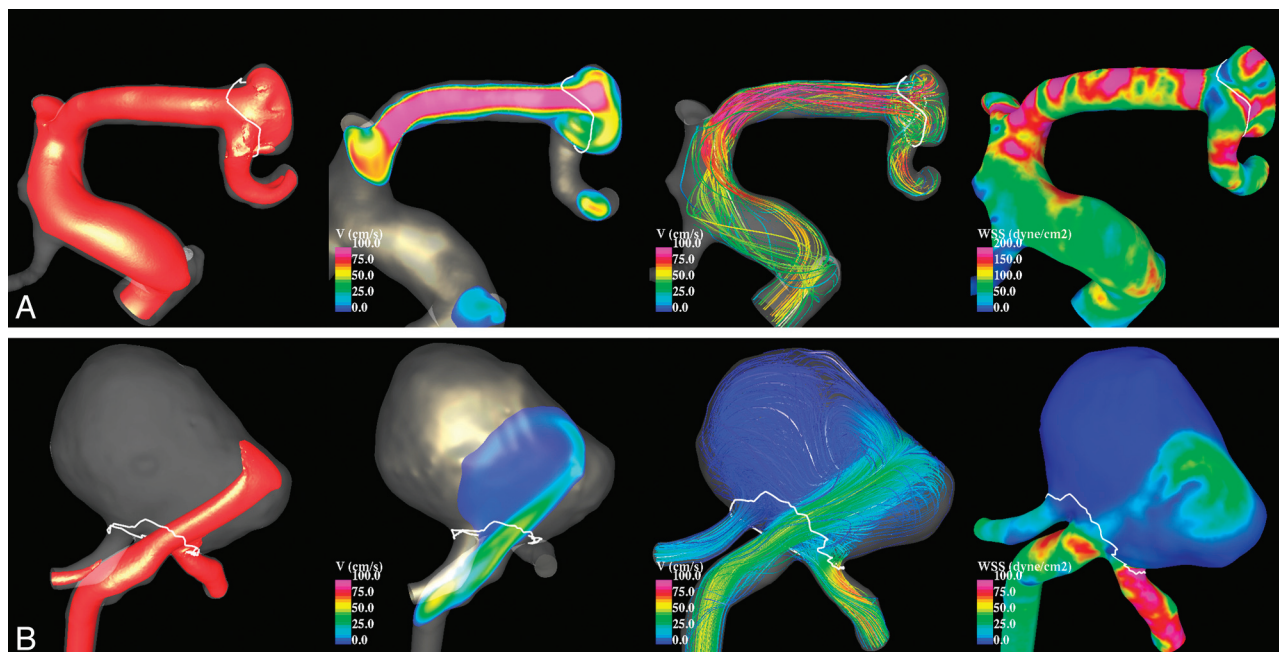
Fig 3. Examples of aneurysms with large (top) and small (bottom) impingement regions. From left to right, the visualizations show isovelocity surfaces, velocity magnitudes on a cut plane, streamlines, and WSS distribution, all at peak systole.
