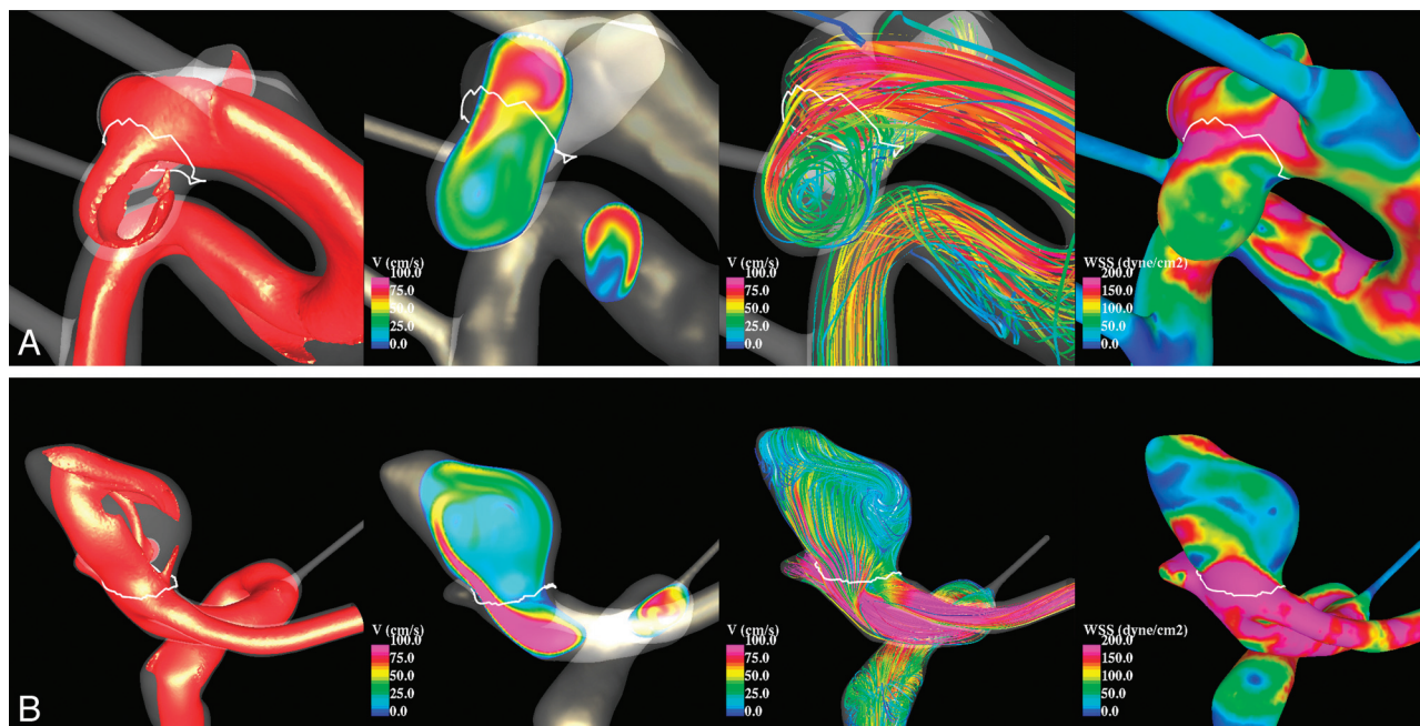
Fig 1. Examples of aneurysms with simple (top) and complex (bottom) flow patterns. From left to right, the visualizations show isovelocity surfaces, velocity magnitudes on a cut plane, streamlines, and WSS distribution, all at peak systole.
