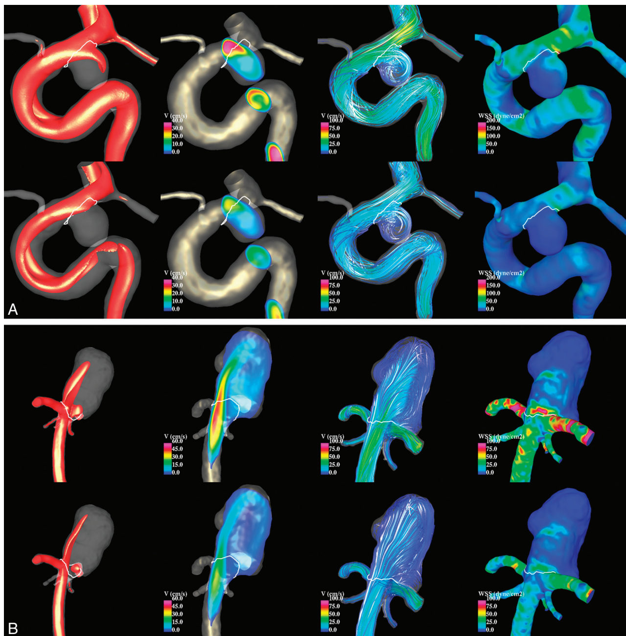
Fig 2. Examples of aneurysms with stable (top) and unstable (bottom) flow patterns. Visualizations at peak systole (top row of each panel) and end diastole (bottom row of each panel) are shown by using (from left to right) isovelocity surfaces, velocity magnitudes on a cut plane, streamlines, and WSS distribution.
