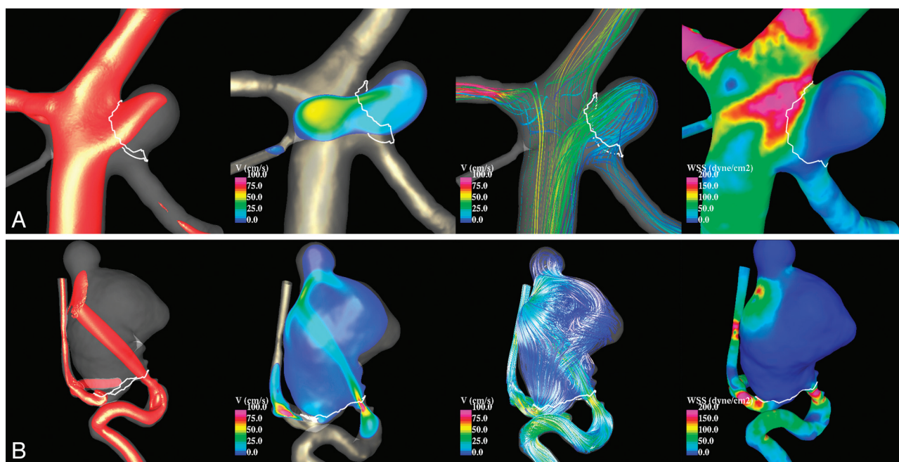
Fig 4. Examples of aneurysms with diffuse (top) and concentrated (bottom) inflows. From left to right, the visualizations show isovelocity surfaces, velocity magnitudes on a cut plane, streamlines, and WSS distribution, all at peak systole.
