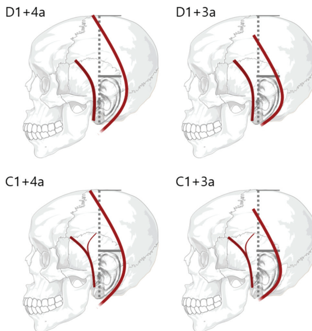
FIG 3. PAA-EDAS candidates.
