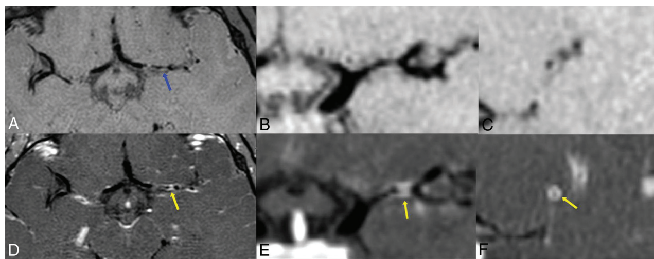
FIG 2. Vessel wall enhancement within the M1 left MCA. Vessel wall imaging targeted to the left middle cerebral artery with axial pre- (A) and postcontrast (D) 3D T1 volume isotropic turbo spin-echo acquisition sequences, with reformatted coronal images (B and E, respectively). Pre- (C) and postcontrast (F) reformatted sagittal images en face to the M1 left middle cerebral artery at the level of the blue and yellow arrows, respectively. There is wall thickening ( blue arrow ) and marked concentric contrast enhancement of the M1 left middle cerebral artery at the segment of stenosis ( yellow arrows ). The imaging findings, in conjunction with the clinical history, were consistent with FCA-inflammatory type.
