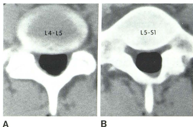
Fig. 1.—Normal case. Air CT at L4-L5 (A) and L5-S1 (B) disk levels. Air fills subarachnoid space and abuts posterior margins of disks. Root sleeves are not visualized.
