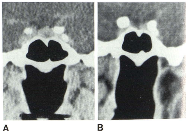
Fig. 3.—Pre- (A) and post- (B) bromocriptine treatment of pituitary microadenoma in patient with amenorrhea galactorrhea. A, Small upward bulging of pituitary gland and diaphragma with slight radiolucency of tumor region. B, Pituitary fossa contents are diminished with partly empty sella.
