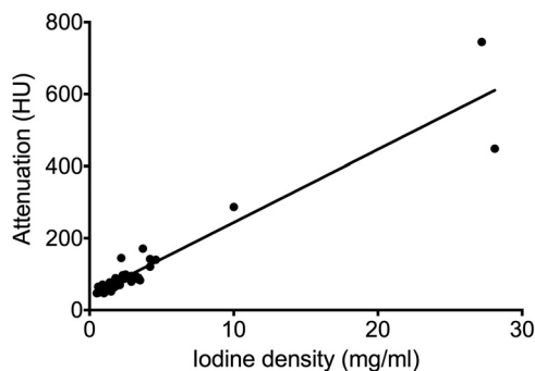
FIG 5. Graph showing the linear correlation existing between maximum hyperdense attenuation and maximum iodine concentration.
