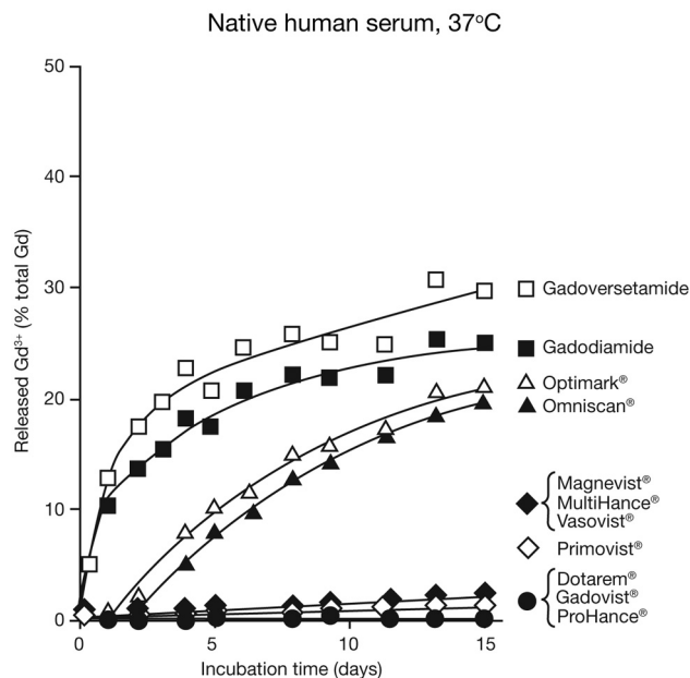
Fig 3. Comparison of rates of Gd^{3+} release for 1 mmol/L solutions of gadolinium-containing contrast agents in native human serum from healthy volunteers at 37°C. Reprinted with permission from Frenzel T, Lengsfeld P, Shirmer H, et al. Stability of gadolinium-based magnetic resonance imaging contrast agents in human serum at 37°C. Invest Radiol 2008;43:817–28.
