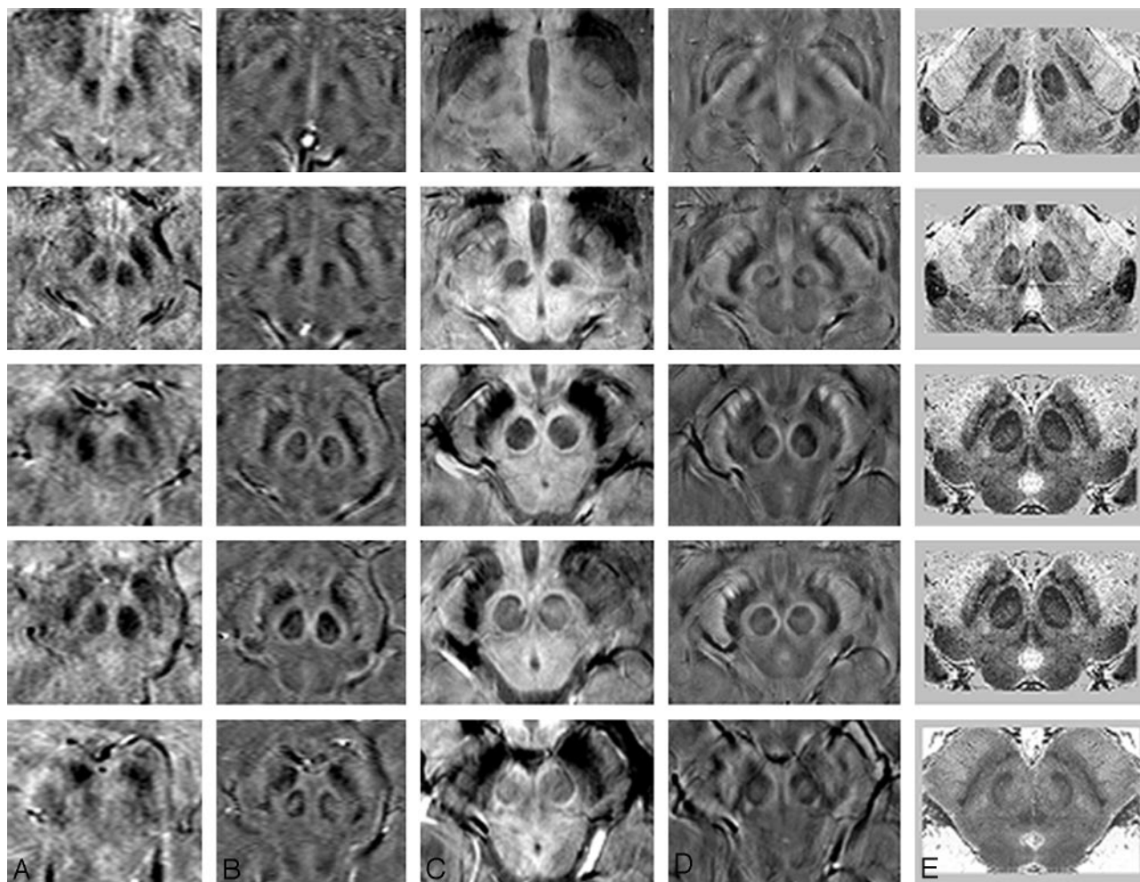
Fig 3. A comparison of adjacent sections in SWI magnitude and HP-filtered-phase images at 1.5T and 4T with Duvernoy's india ink-stained results. 16 A , Magnitude SWI at 1.5T; B , HP-filtered phase at 1.5T; C , Magnitude SWI at 4T; D , HP-filtered phase at 4T; E , Duvernoy's results. Only 3 unique images from Duvernoy are shown here because his section thickness is 3 mm. The third and fourth images from the top are identical. Images in column E reprinted with permission from Duvernoy HM. Human Brain Stem Vessels . 2nd ed. Berlin, Germany: Springer-Verlag; 1999:206–13.
