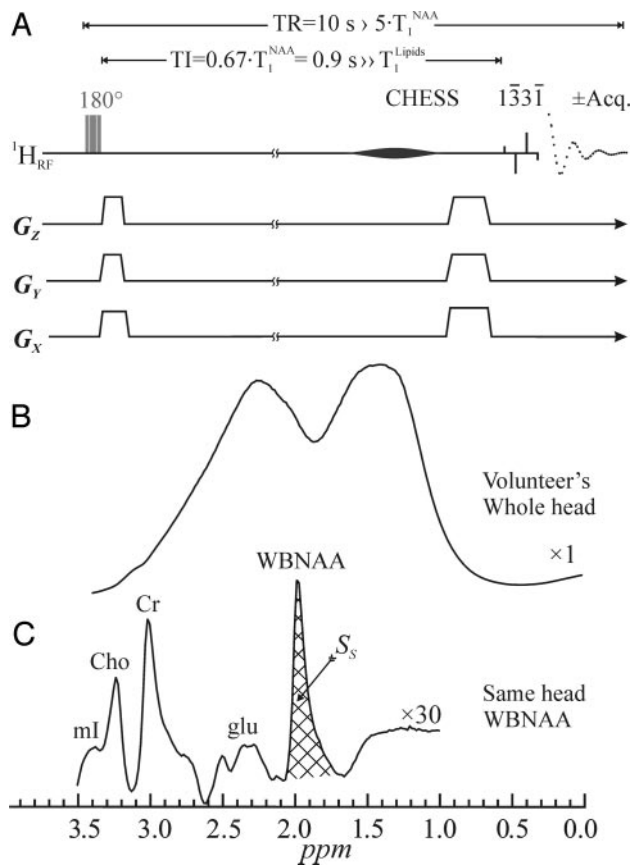
Fig 3. Top: A, Schematic representation of the 2-step WBNA sequence. It comprises an alternating inversion pulse (applied every odd acquisition) followed by a TI designed to null the NAA signal. It ends with a chemical-shift-selective (CHES) and a ^{133}\text{I} water-suppression pulse (4-ms interpulse delay at 1.5T). The latter also serves as the 90° readout pulse. Acquisition commences immediately ( \text{TE} = 0 ), and every even acquisition is subtracted from every odd one. Because the TR is long, 10 seconds, no T1- or T2-weighting is incurred. Note that all the radio-frequency (RF) pulses are (spatially) nonselective and the gradient “blips” are just crushers. Center: B, The result of a 90° ^{133}\text{I} on a human head, demonstrating the problem of the immense metabolite-observing lipid signal from the bone marrow and adipose tissue. Bottom: C, The resulting spectrum from the WBNA sequence on the same head as in B, demonstrating almost complete lipid suppression. Note that the NAA is implicitly localized to the brain, whereas with the other metabolites whose peaks are distinct and nonlocalized, it is impossible to ascertain where their signals come from. Also note the excellent SNR from this 2.5-minute acquisition.
