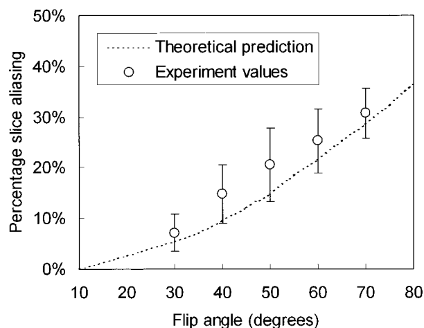
FIG 3. Percentage section aliasing, calculated as widening of the full-width-at-half-maximum of the steady-state signal intensity profile relative to the desired slab thickness, plotted as a function of the designated flip angle (dotted line). Experimental measurements (circles) from our subjects agreed fairly well with the theoretical deductions. Note that, at a 70° flip angle, the percentage section aliasing is nearly 30%, meaning that about one-third of the sections would be subject to interference from CSF outside the image slab. By lowering the flip angle to 30° or 40°, the percentage section aliasing decreases to <20%.
