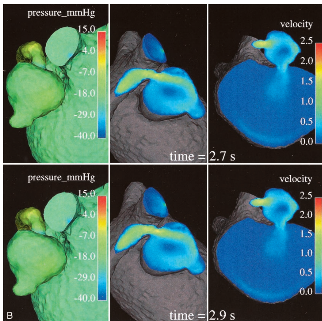
FIG 4. Relative surface pressure maps (left images; in mm Hg) for both aneurysms and MPCa at different time moments of one cardiac cycle show marked pressure variations in the arterial aneurysm caused by the jet coming from the parent artery stenosis. High-pressure areas all over the cardiac cycle are seen opposite of the stenotic artery entry hole. Central and right images demonstrate the blood velocity (magnitude; in m/s) maps in two cross sections and outflow boundary.
