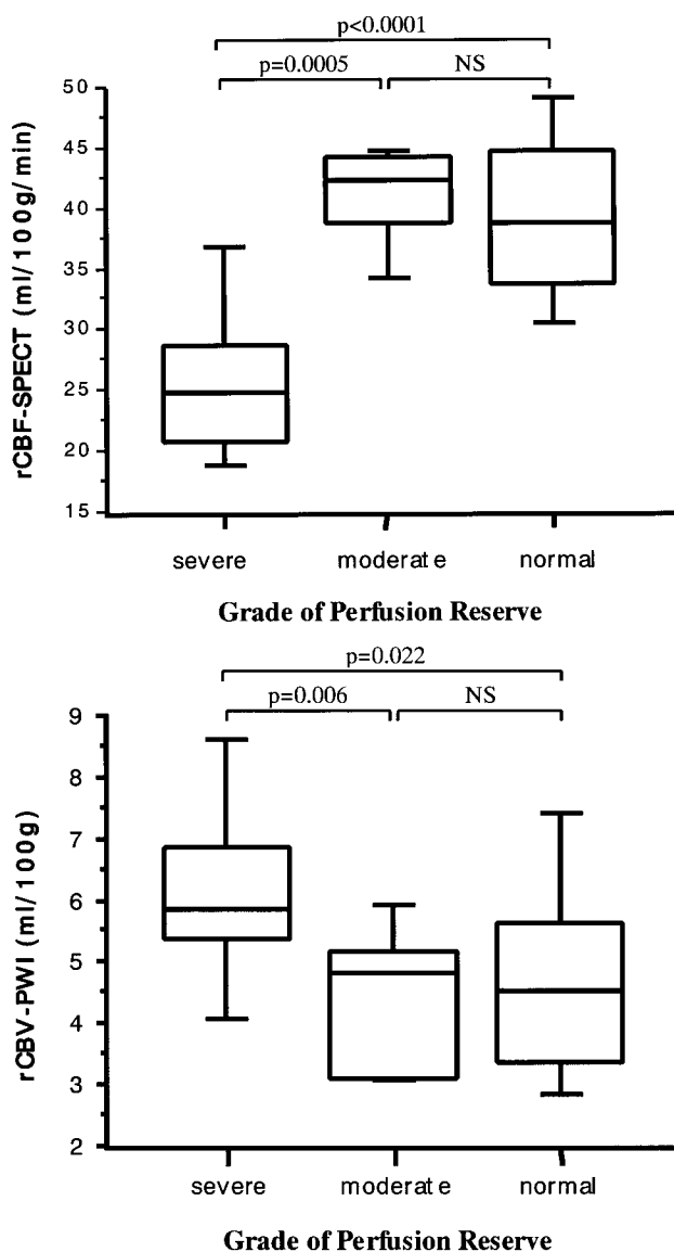
FIG 4. A–C, Box-and-whisker plot of rCBF-SPECT (A), rCBF-PWI (B), and rCBV-PWI (C) in the regions with severely decreased ( 0 < \% \text{ increase} \leq 15\% ), moderately decreased ( 15\% < \% \text{ increase} \leq 15\% ), and normal ( 15\% < \% \text{ increase} ) perfusion reserve. \% \text{ increase} was defined as [(\text{post-rCBF}) - (\text{pre-rCBF})]/(\text{pre-rCBF}) \times 100 , where pre-rCBF and post-rCBF denote the CBF values before and after acetazolamide CBF as measured on ^{133}\text{Xe} -SPECT scans, respectively. Boxes represent 25% to 75% range with bisecting lines showing median values; horizontal lines represent 10% to 90% range; NS indicates not significant. Note that the regions with severely decreased perfusion reserve show significantly lower rCBF values on ^{133}\text{Xe} -SPECT (A) and rCBF-PWI (B) studies than do those with moderately decreased or normal perfusion reserve. They also show significantly higher rCBV values on rCBV-PWI study (C) than do those with moderately decreased or normal perfusion reserve.
