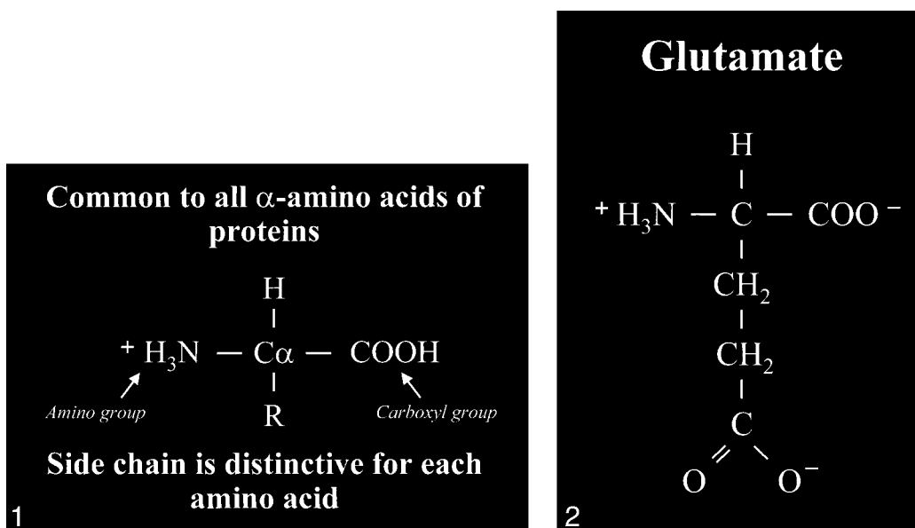
FIG 1. Amino acid. Typical amino acid consists of a central alpha carbon ( \text{C}_\alpha ) that is bonded to a carboxyl group ( \text{COOH} ) on one side and an amino group ( \text{H}_3\text{N} ) on the other side. Each amino acid is characterized by a distinctive molecular group ( \text{R} ) or side chain attached to the \alpha carbon.
