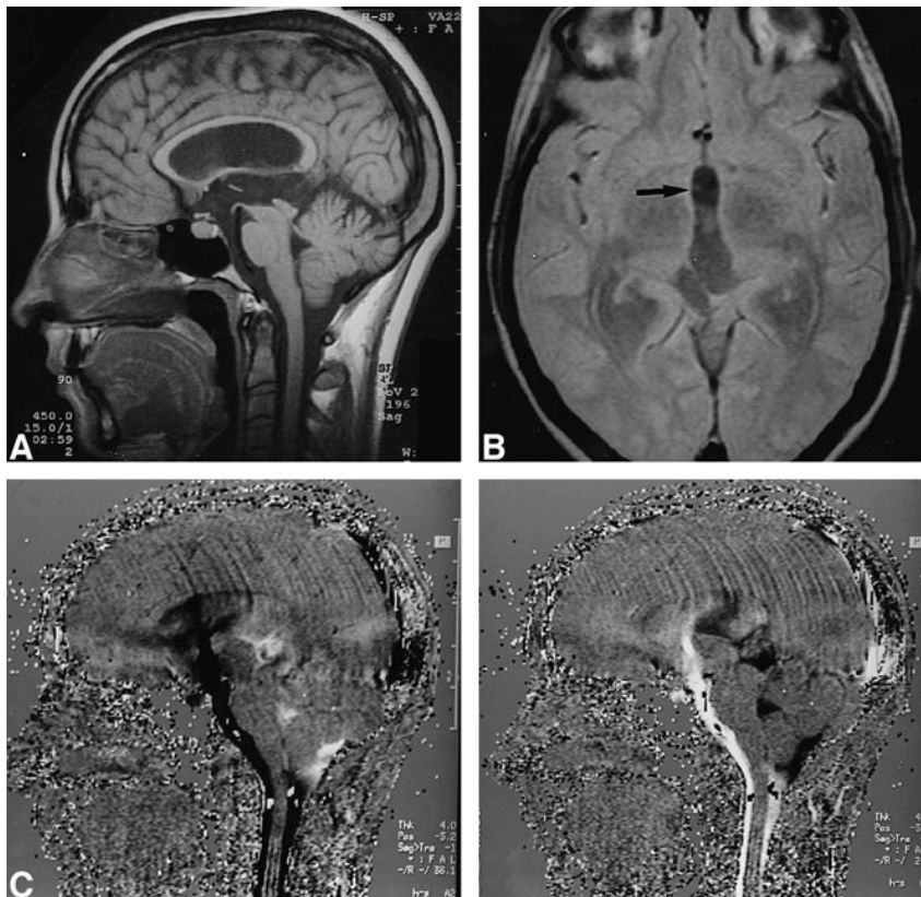
FIG 2. Aqueductal stenosis.
