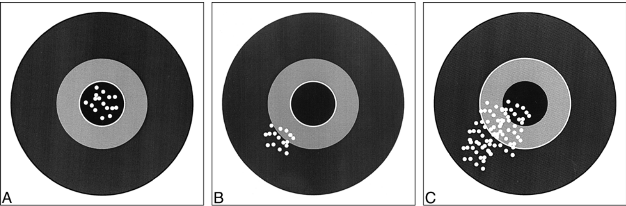
FIG 3. Validity and reliability of a test. A, Good validity and reliability means the center of the target is always hit by different gunmen. B, Good reliability but poor validity means the same area of the target is hit by different gunmen but off center. C, Poor reliability of the test means the bullets are spread out, all over the target, with a few hitting the center. In the hands of a few gunmen a test can be valid, since the center of the target is hit.
