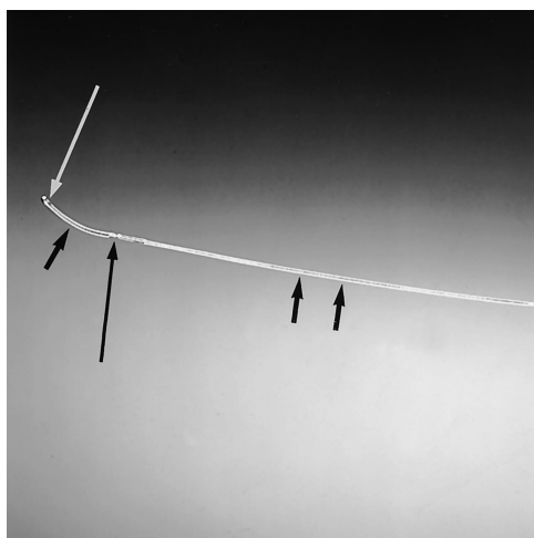
Fig 5. The distal end of the detachable endovascular electrocoagulation device shows stainless steel delivery wire (double arrows); uninsulated steel junction (long black arrow); crescent-shaped 6-mm long platinum coil (short arrow). The distal, 1-mm, portion of the platinum coil is insulated (white arrow) to avoid possible convergence of the RF energy in a too-small area of the vessel.
