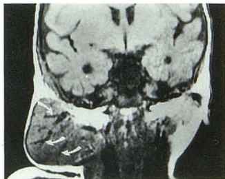
Fig. 2. Four-month-old child with a proliferating hemangioma. Coronal T1-weighted image (600/20) demonstrates an intermediate signal intensity mass containing vascular flow voids (arrows).
