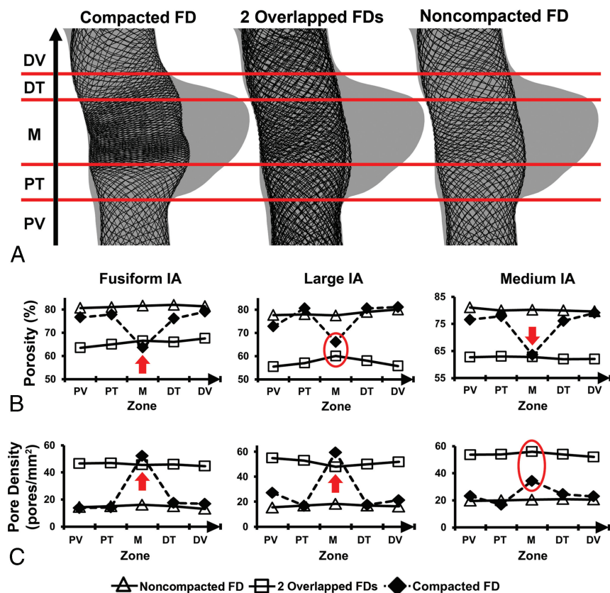
FIG 2. Porosity and pore density distributions of deployed FDs resulting from all 3 deployment methods in the 3 IAs. A, Deployed FD meshes in the fusiform IA and demarcations of FD zones used for porosity and pore density calculations: proximal vessel (PV), proximal transition (PT), middle (M), distal transition (DT), and distal vessel (DV). These zones are defined on the basis of the compacted FD but applied to all 3 deployment strategies for calculation of porosity and pore density. B, Porosity distribution. C, Pore density distribution. The arrows indicate middle zones in which the compacted FD has lower porosity or higher pore density than the overlapped FDs, whereas the ovals indicate middle zones in which it does not.
