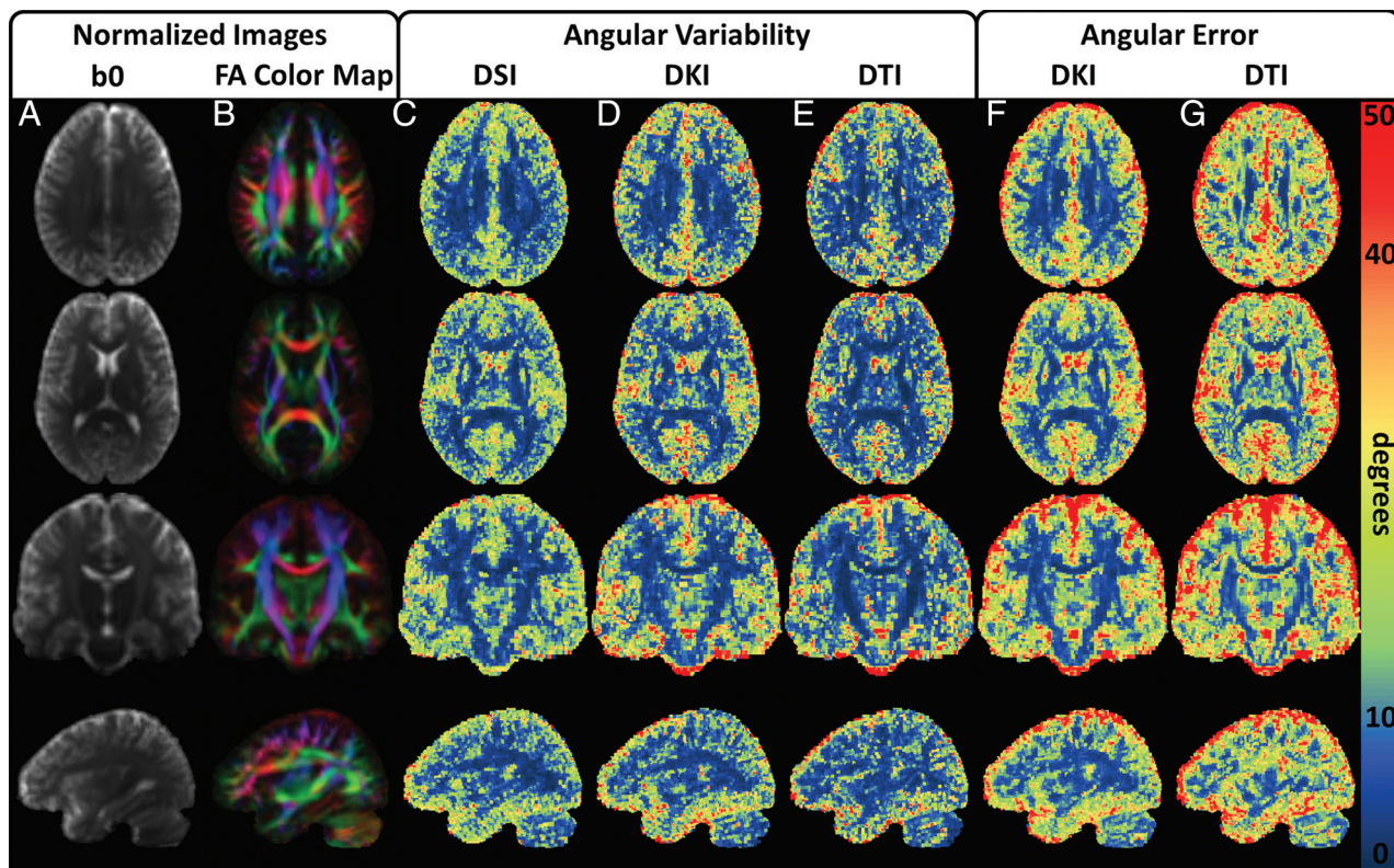
FIG 3. Group mean angular variability and angular error maps illustrate dODF performance. A and B, Mean of the normalized b0 and FA color map images, respectively, from all DKI acquisitions. These are included for anatomic reference and to help validate the normalization procedure. The rows illustrate representative transverse, coronal, and sagittal orientations. C–E, Angular variability for the DSI, DKI, and DTI reconstructions, respectively. All 3 techniques demonstrate similar angular variability in the white matter regions. F and G, Angular error for the DKI and DTI reconstructions, respectively. Angular error measures increase in regions with low FA, though the angular error for the DKI reconstruction is relatively consistent throughout the WM. The angular error is higher for the DTI reconstruction in the WM, particularly in regions where complex fiber bundle geometries may be present.
