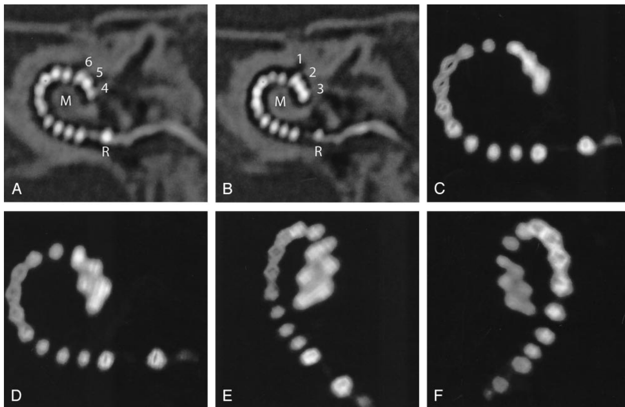
FIG 2. Case 1. A and B, Oblique MPRs of high-resolution MSCT images in the plane of the electrode array demonstrate 16 electrode contacts within the scala tympani. The tip of the electrode (contacts 1–3) projects cranial to contacts 4–6, indicating kinking of the electrode array. C–F, 3D VR images confirm this finding. On conventional radiography (cochlear view) electrode contacts 1–6 would be superimposed on each other, as compared with image 2C. R indicates reference electrode; M, modiolus.
