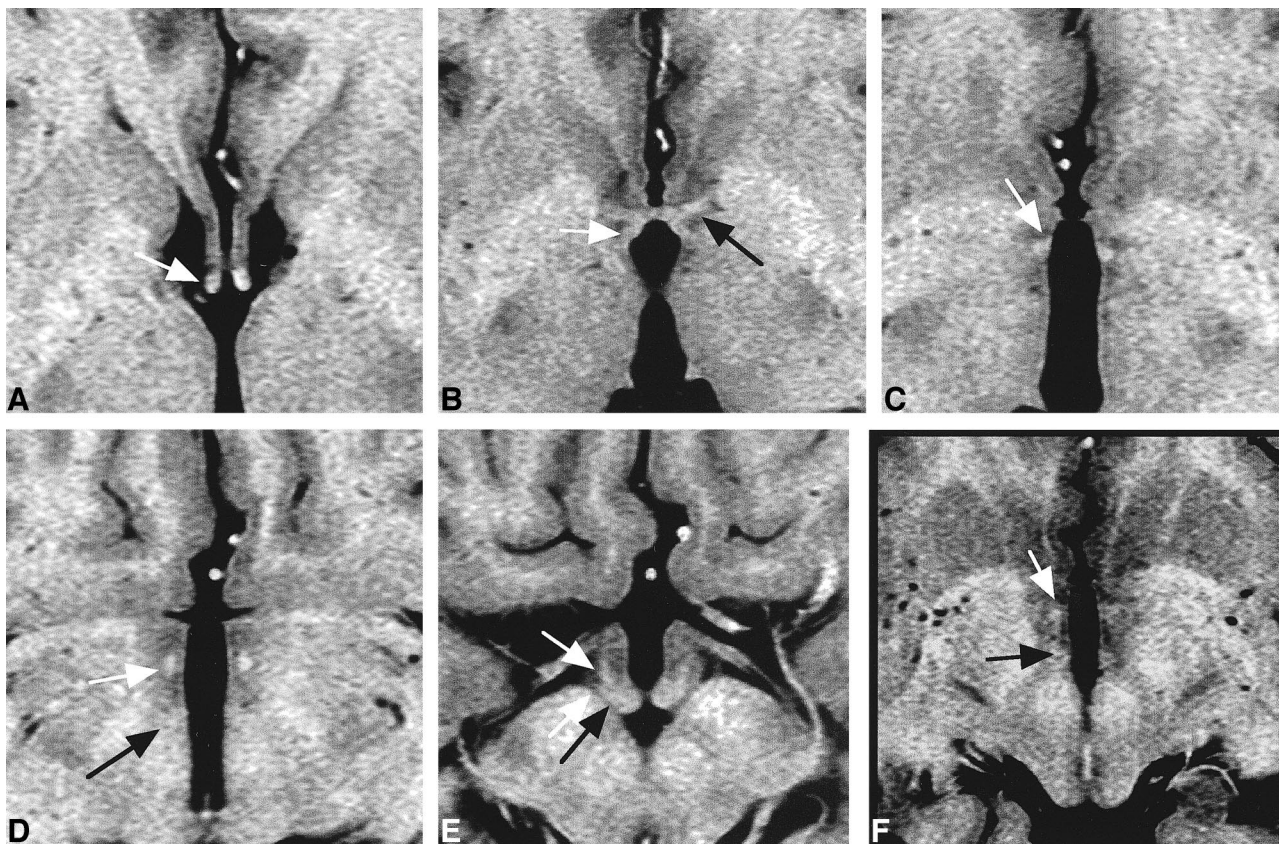
FIG 2. Axial images of consecutive five sections in one healthy subject shown in Figure 1 (A–E) and one section in another subject (F). A, Fornical columns (arrow) were observed in one section level above the anterior commissure. B, PF (white arrow) was observed as a high-signal-intensity spot just behind the anterior commissure (black arrow) and exposed to the cerebrospinal fluid space of the third ventricle. C, In the next lower section, PF (arrow) was still exposed to the third ventricle. D, In the next lower section, ovoid PF (white arrow) directing posteriorly toward the mammillary body was seen. Ill-defined high-signal-intensity spot (MT; black arrow) was visible 4 mm posterior to PF. E, At the next level, PF (white arrow) joined to the mammillary body (black arrow) anteriorly and laterally. F, PF (white arrow) was visible but ill-defined bilaterally. Obscure PF was seen in 6% of healthy subjects. MT (black arrow) was identifiable in this case.
