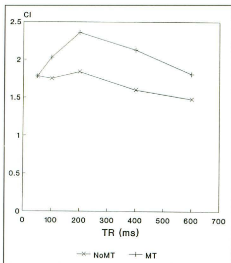
Fig 2. Contrast index (CI) between tumor and edema on Gd-enhanced images without (NoMT) and with (MT) magnetization transfer effect as a function of the TR. Contrast index is expressed as a mean value of four cases. The length of the magnetization transfer pulse is TR -40 milliseconds.
