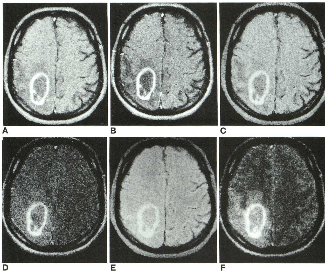
Fig 4. Glioblastoma multiforme. The Gd-enhanced images display ring enhancement, cystic or necrotic centers, and surrounding nonenhancing tumor or edema.
